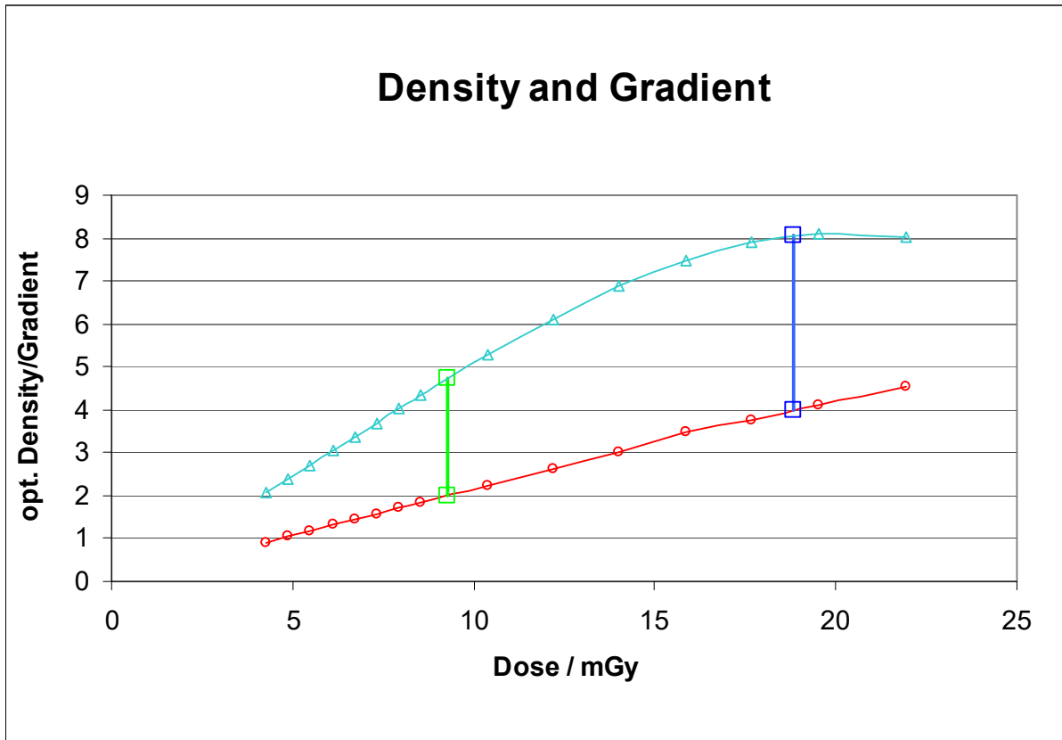
Figure 1: Mean optical density \langle D-D_0 \rangle (red curve) and mean gradient \langle G \rangle (blue curve) of eight films as function of exposure dose K (Reg. No. BAM 17-19).
