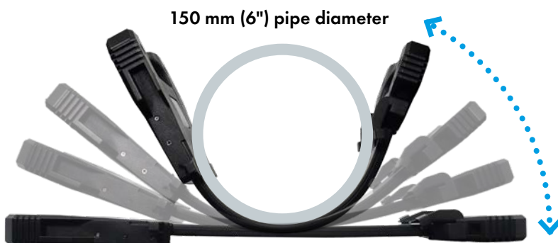
The D-DR 1025B NDT can be bent continuously from flat to a 150 mm diameter in one direction, the D-DR 1043B NDT to a 300 mm diameter.
